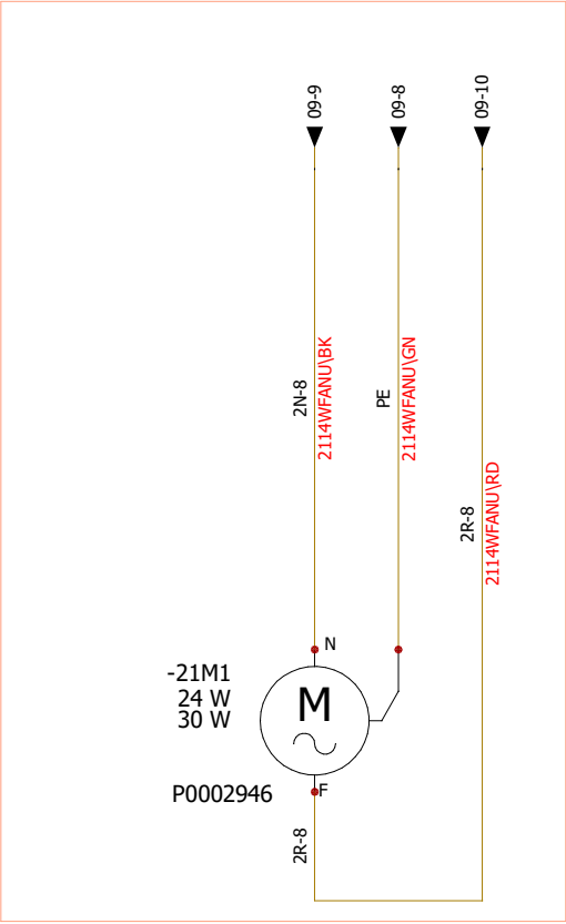
+2+2.1 - Electrical Plate
