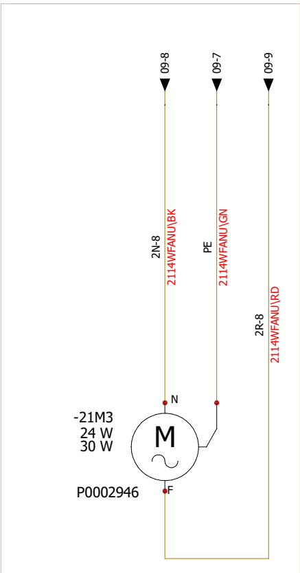
+2+2.1 - Electrical Plate
