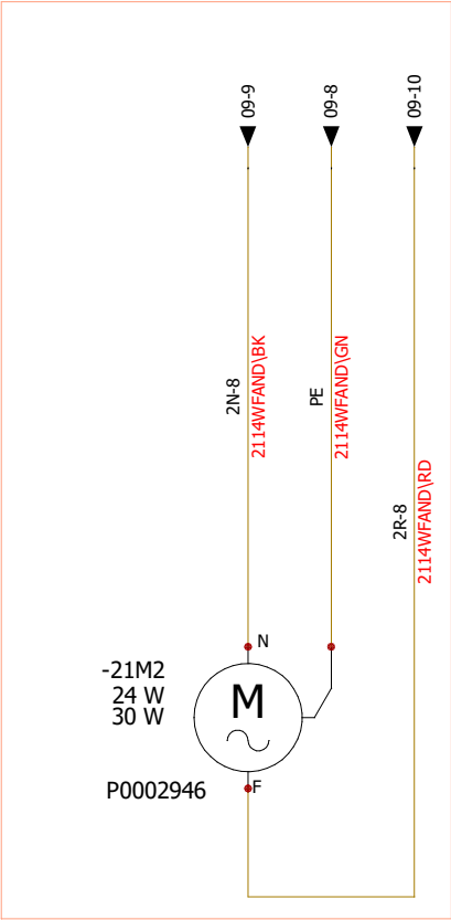
+2+2.1 - Electrical Plate
