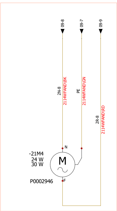
+2+2.1 - Electrical Plate
